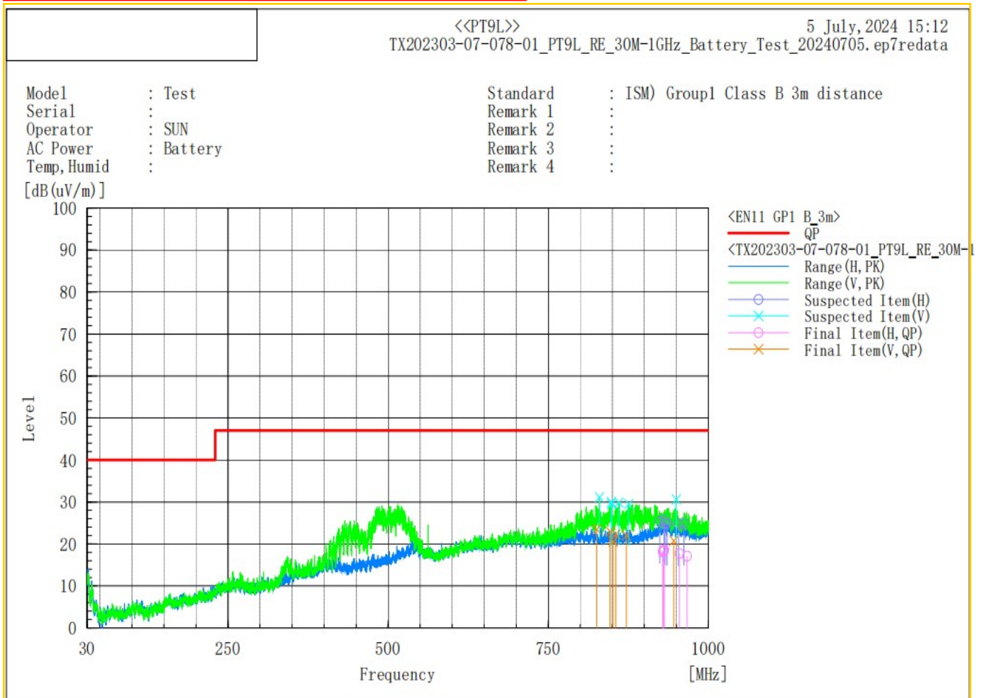
Figure 2: Measurement results of radiated emission, Mode 2
