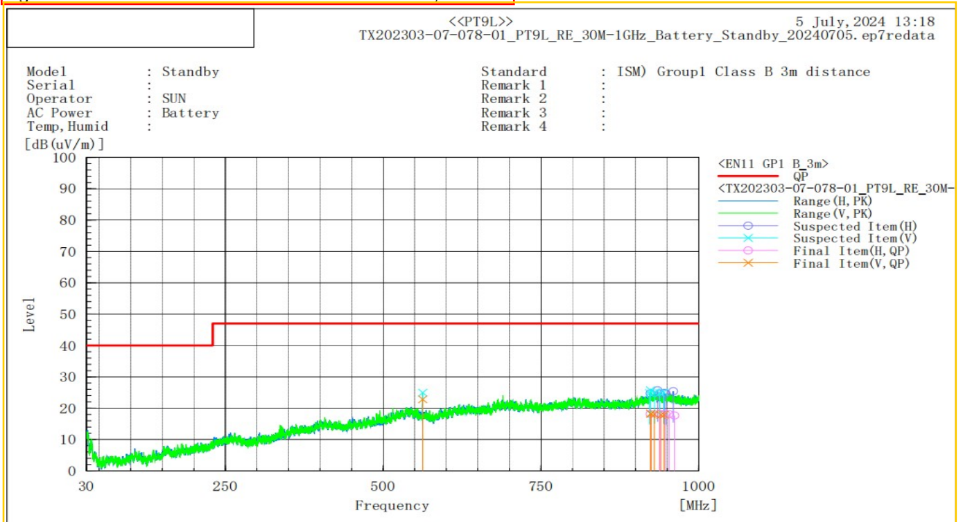
Figure 1: Measurement results of radiated emission, Mode 1
